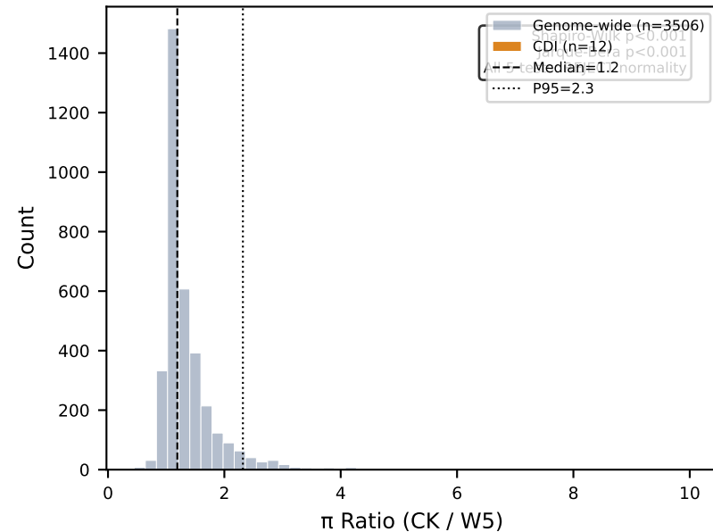
A: \pi Ratio Distribution — Chr05 (100-kb windows)
