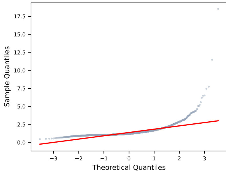
B: Q-Q Plot — Severe Deviation from Normal
