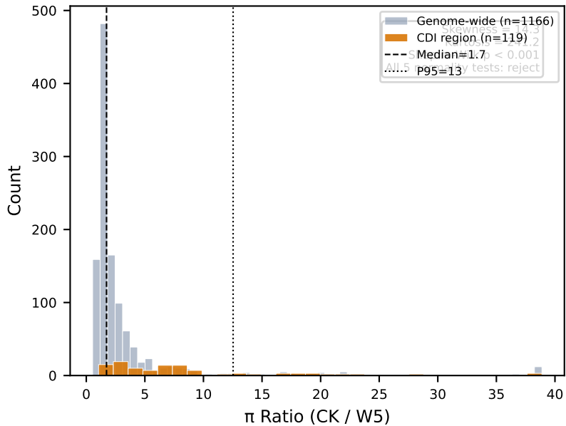
A: Distribution of \pi Ratio on Chr05
