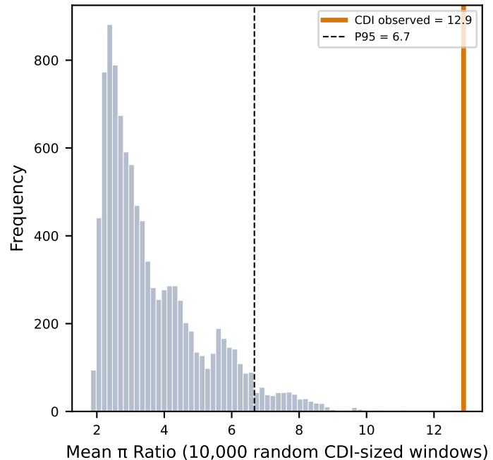
B: Monte Carlo Permutation — p < 0.0001
