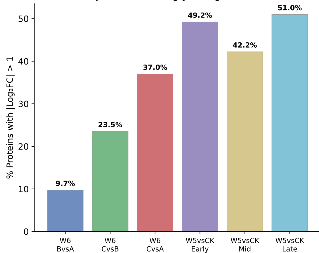
Proportion of Strongly Changed Proteins
