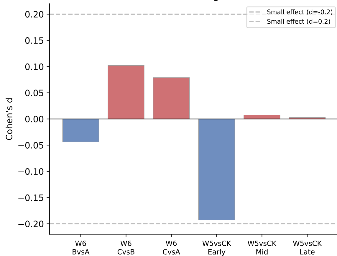
Effect Size (Global Log 2 FC vs Zero)
